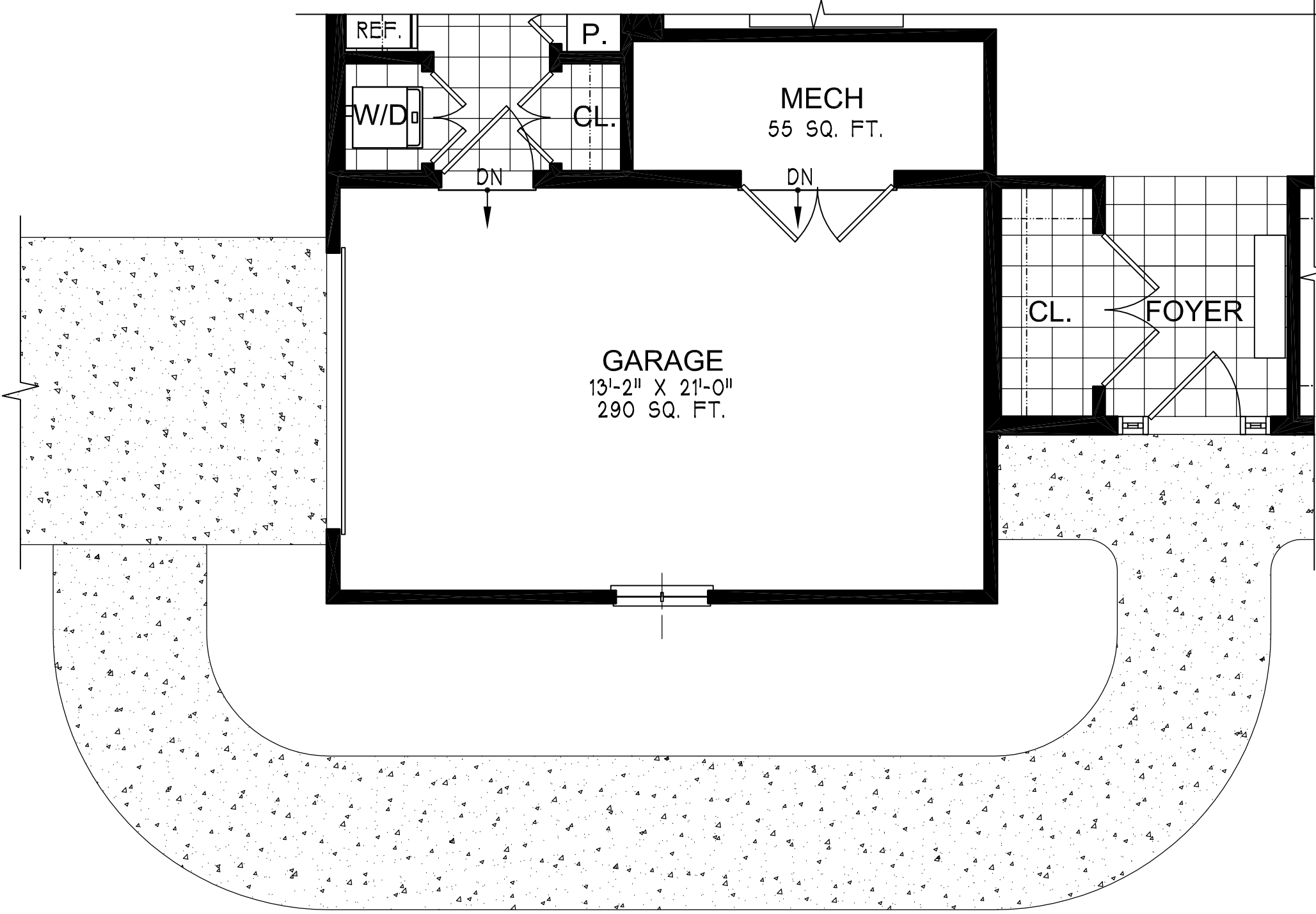
Alternate Garage - Unit 33
